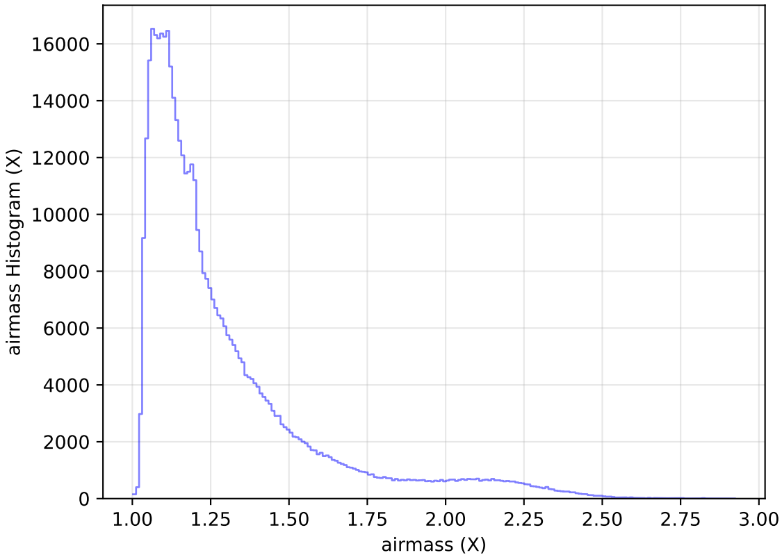
too_elab_r64_d3_gz_v3.4_10yrs WFD r band: airmass Histogram
