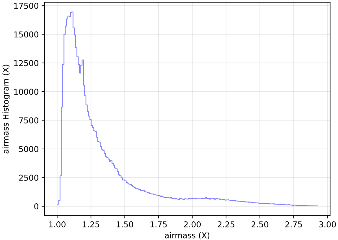
too_elab_r64_d3_gz_v3.4_10yrs WFD i band: airmass Histogram
