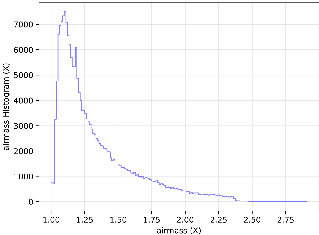
too_elab_r64_d3_gz_v3.4_10yrs WFD g band: airmass Histogram
