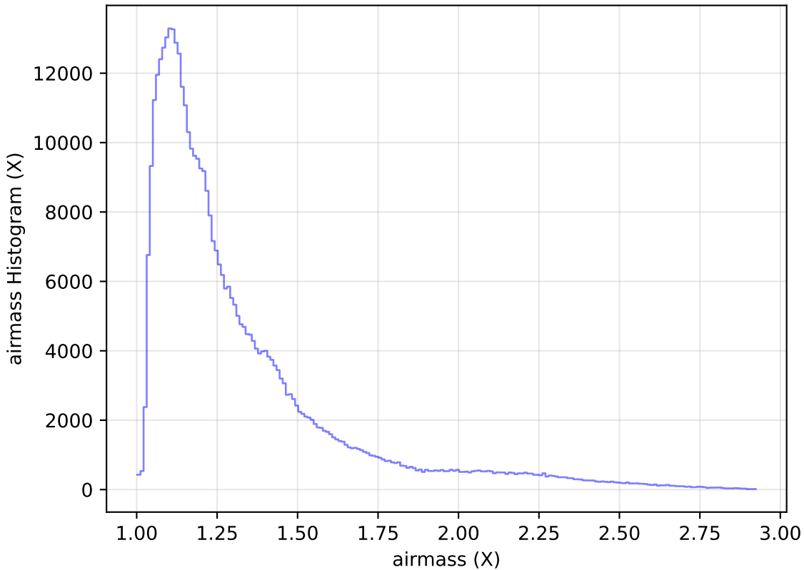
too_elab_r64_d3_gz_v3.4_10yrs All sky z band: airmass Histogram
