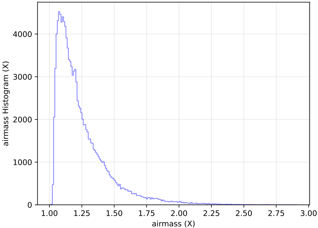
too_elab_r64_d3_gz_v3.4_10yrs All sky u band: airmass Histogram
