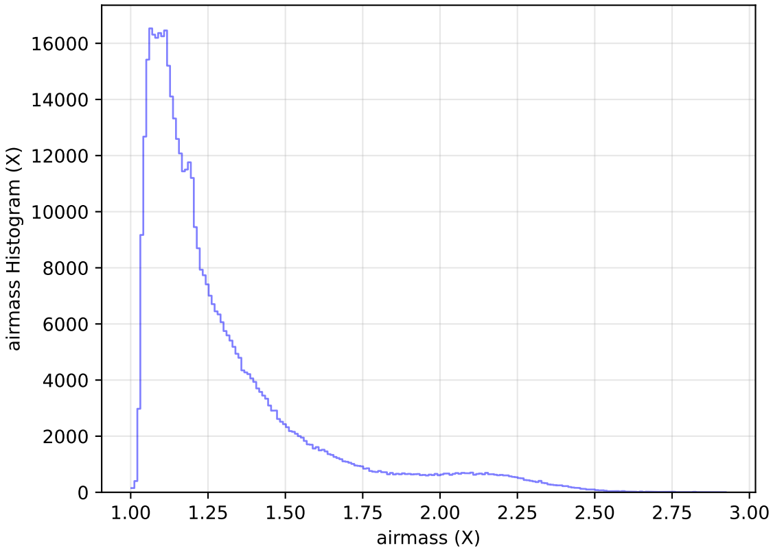
too_elab_r64_d3_gz_v3.4_10yrs All sky r band: airmass Histogram
