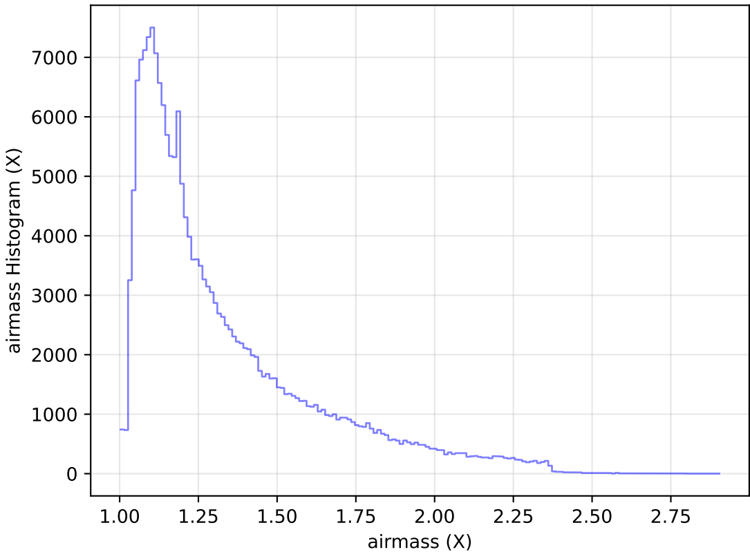
too_elab_r64_d3_gz_v3.4_10yrs All sky g band: airmass Histogram
