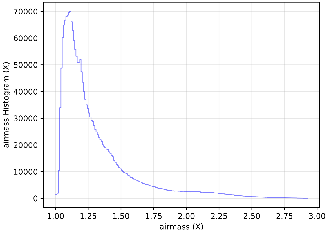
too_elab_r64_d3_gz_v3.4_10yrs All sky all bands: airmass Histogram
