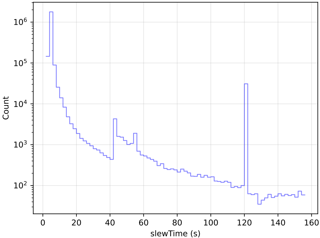
too_elab_r64_d3_gz_v3.4_10yrs All visits: Slew Time Histogram
