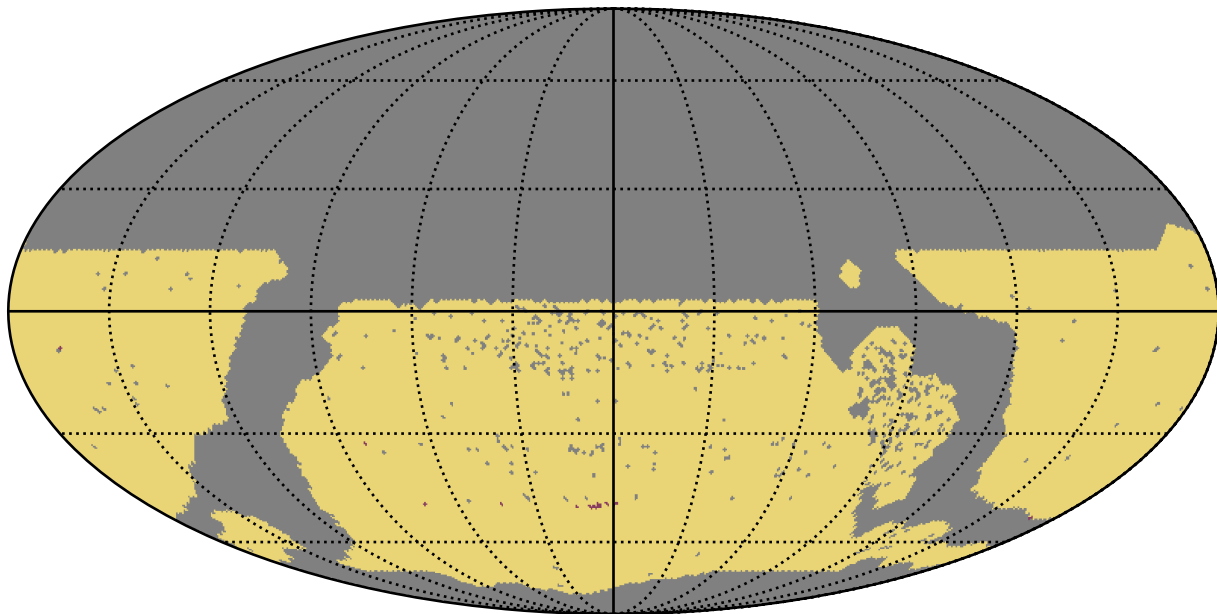
too_elab_r64_d3_gz_v3.4_10yrs WFD: RapidRevisits
