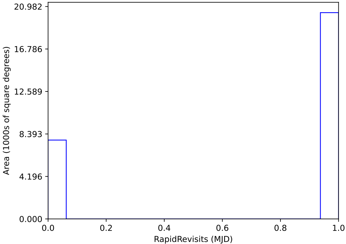
too_elab_r64_d3_gz_v3.4_10yrs All sky: RapidRevisits
