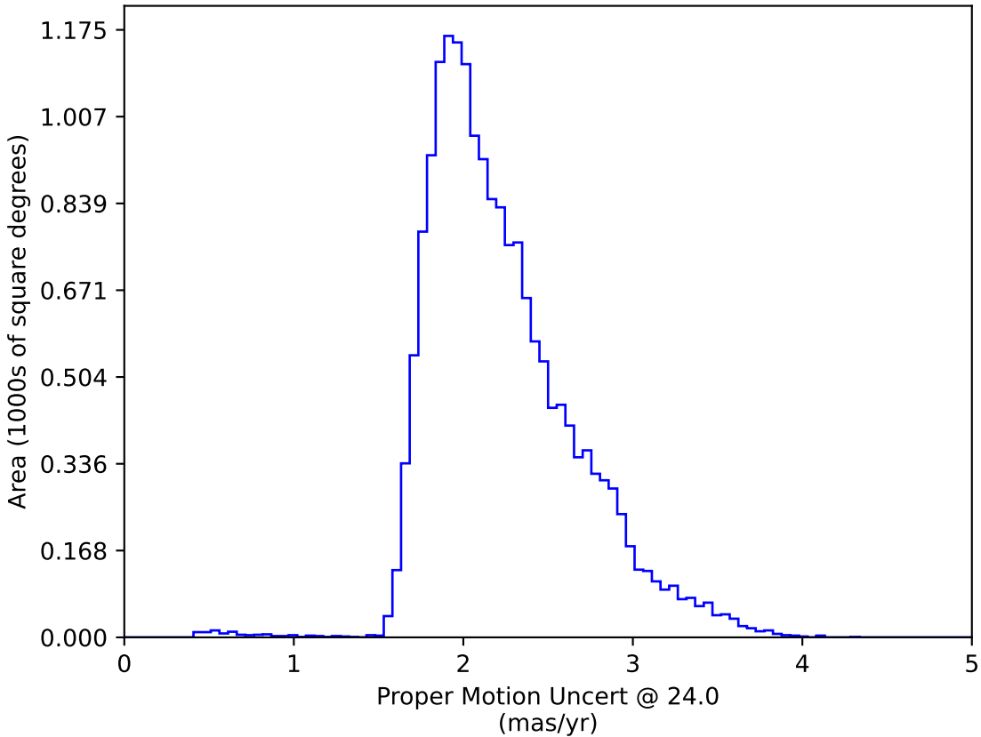
too_elab_r64_d3_gz_v3.4_10yrs WFD: Proper Motion Uncert @ 24.0
