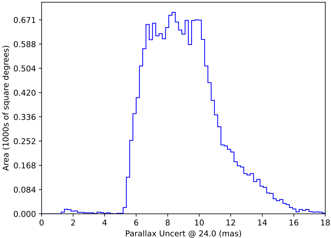
too_elab_r64_d3_gz_v3.4_10yrs WFD: Parallax Uncert @ 24.0
