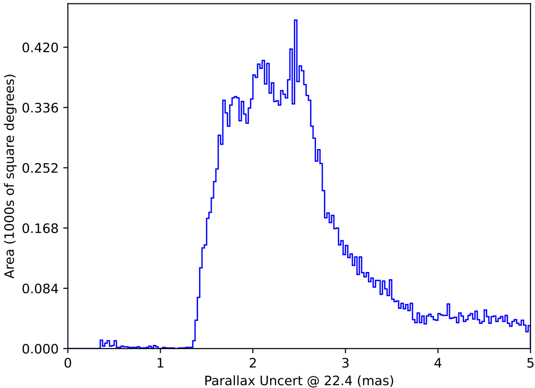
too_elab_r64_d3_gz_v3.4_10yrs All sky: Parallax Uncert @ 22.4
