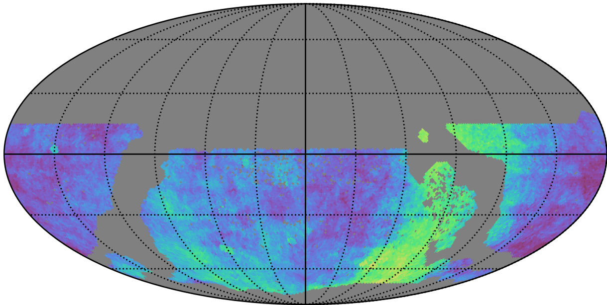
too_elab_r64_d3_gz_v3.4_10yrs WFD: Parallax Coverage @ 24.0
