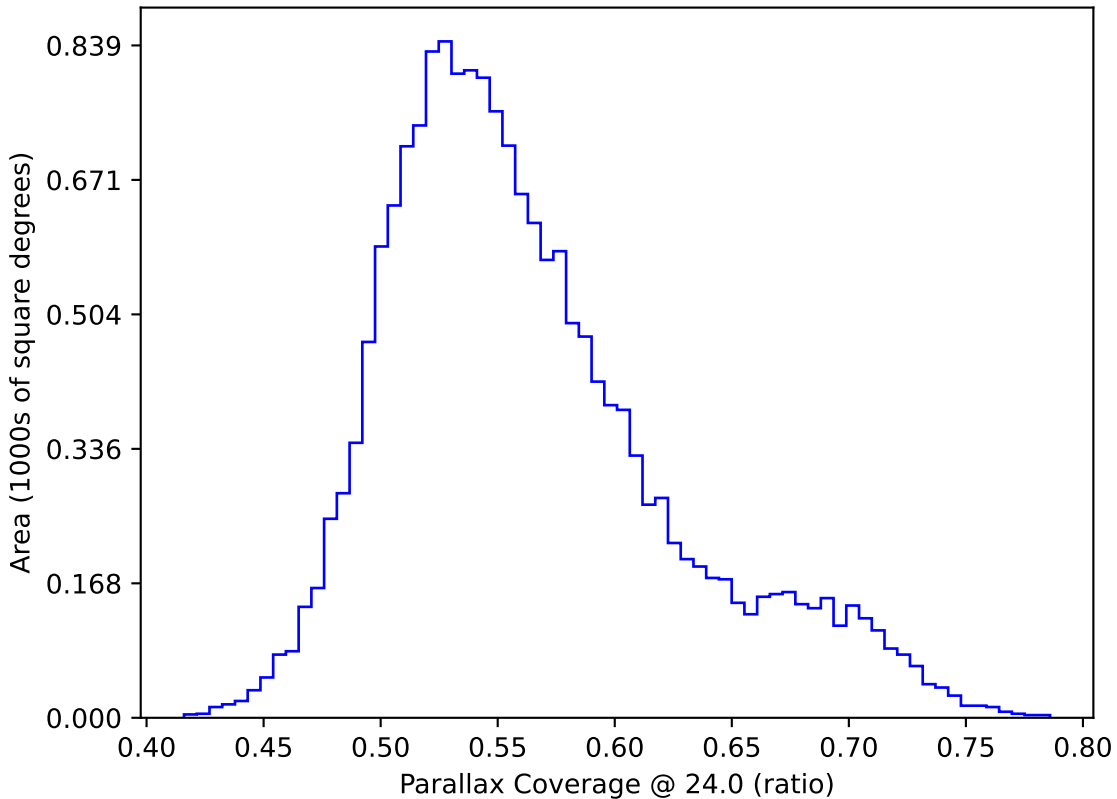
too_elab_r64_d3_gz_v3.4_10yrs WFD: Parallax Coverage @ 24.0
