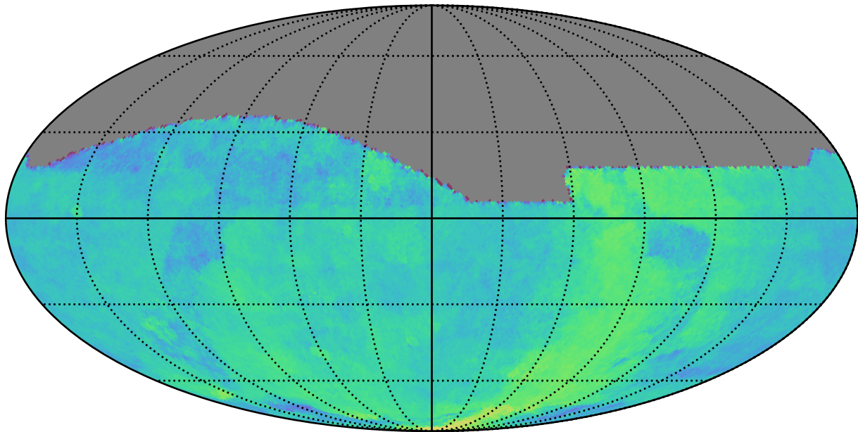
too_elab_r64_d3_gz_v3.4_10yrs All sky: Parallax Coverage @ 24.0
