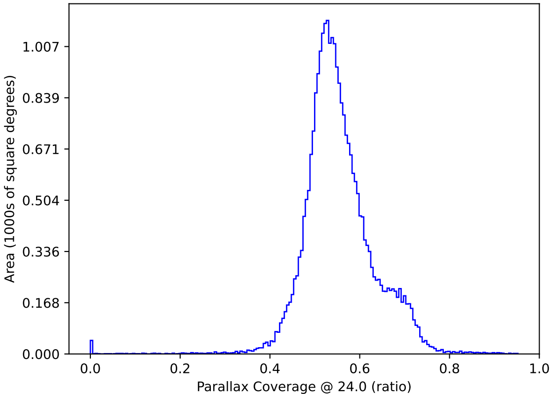
too_elab_r64_d3_gz_v3.4_10yrs All sky: Parallax Coverage @ 24.0
