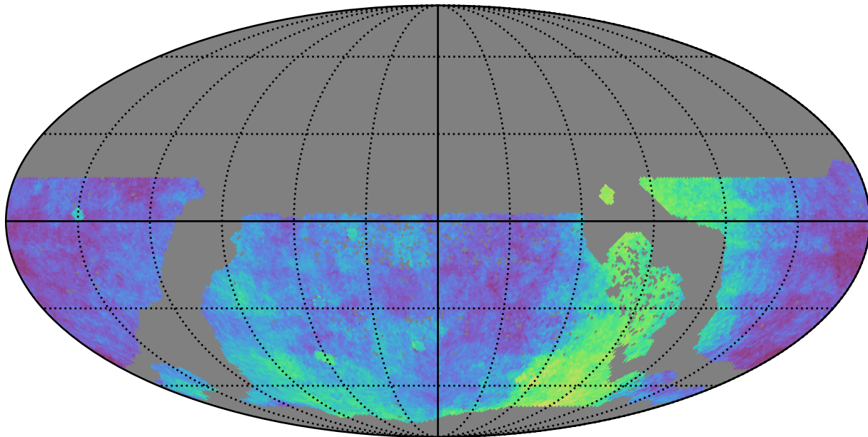
too_elab_r64_d3_gz_v3.4_10yrs WFD: Parallax Coverage @ 22.4
