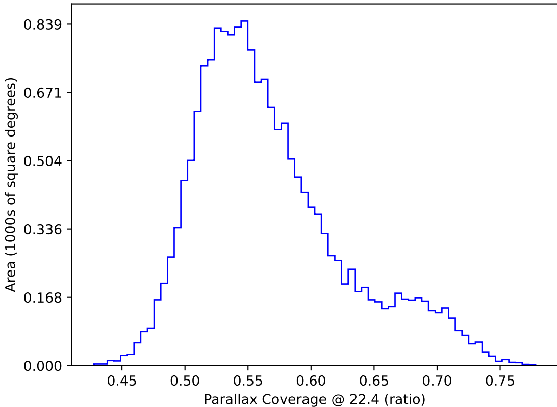
too_elab_r64_d3_gz_v3.4_10yrs WFD: Parallax Coverage @ 22.4
