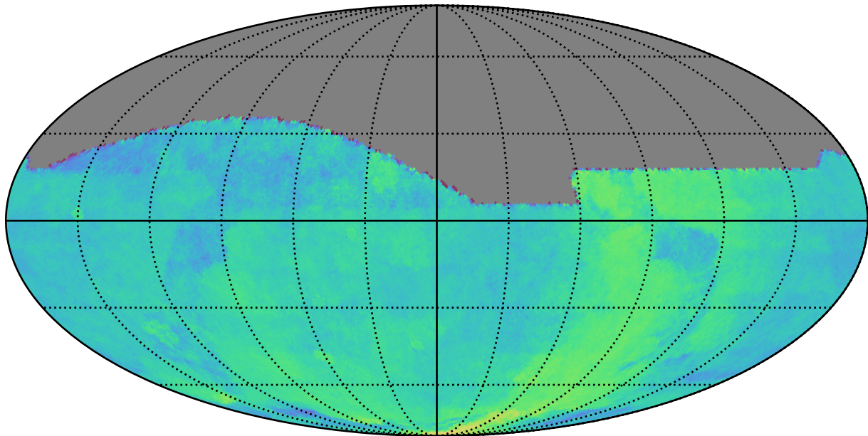
too_elab_r64_d3_gz_v3.4_10yrs All sky: Parallax Coverage @ 22.4
