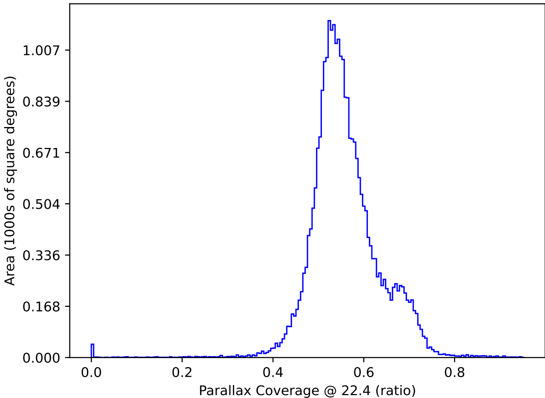
too_elab_r64_d3_gz_v3.4_10yrs All sky: Parallax Coverage @ 22.4
