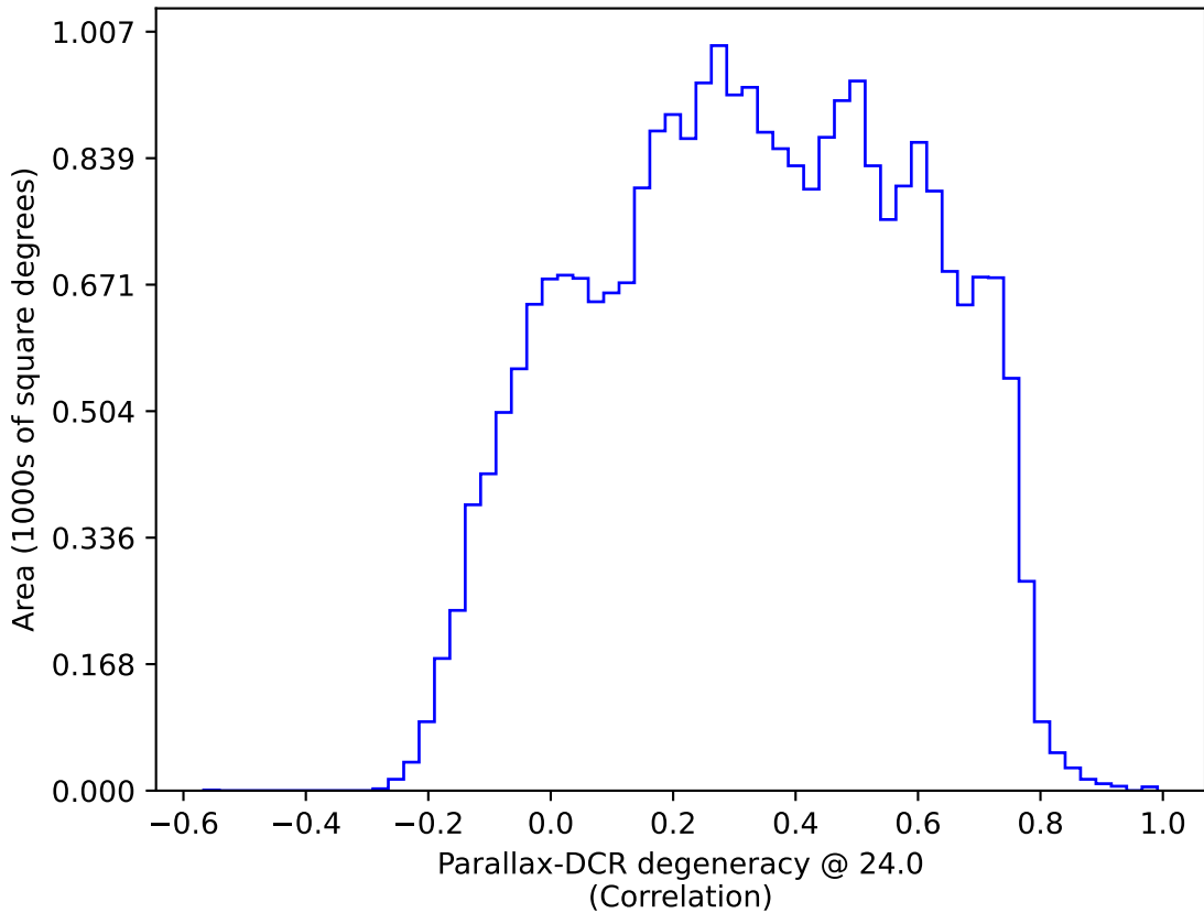
too_elab_r64_d3_gz_v3.4_10yrs All sky: Parallax-DCR degeneracy @ 24.0
