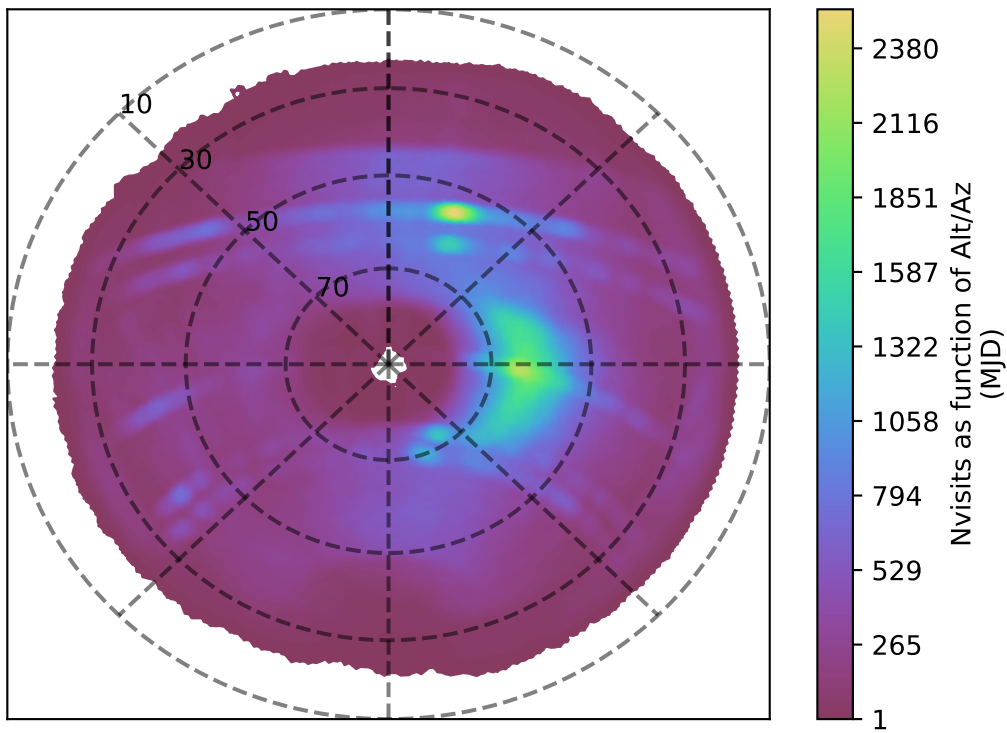
too_elab_r64_d3_gz_v3.4_10yrs z band: Nvisits as function of Alt/Az
