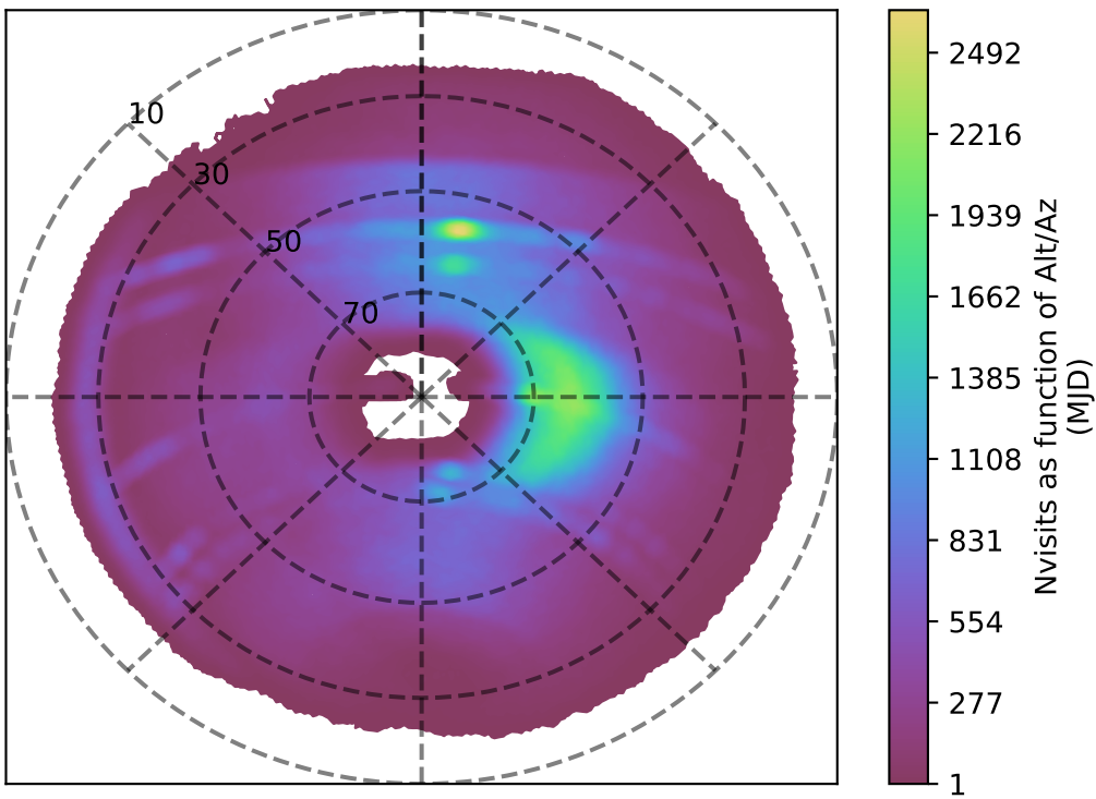
too_elab_r64_d3_gz_v3.4_10yrs r band: Nvisits as function of Alt/Az
