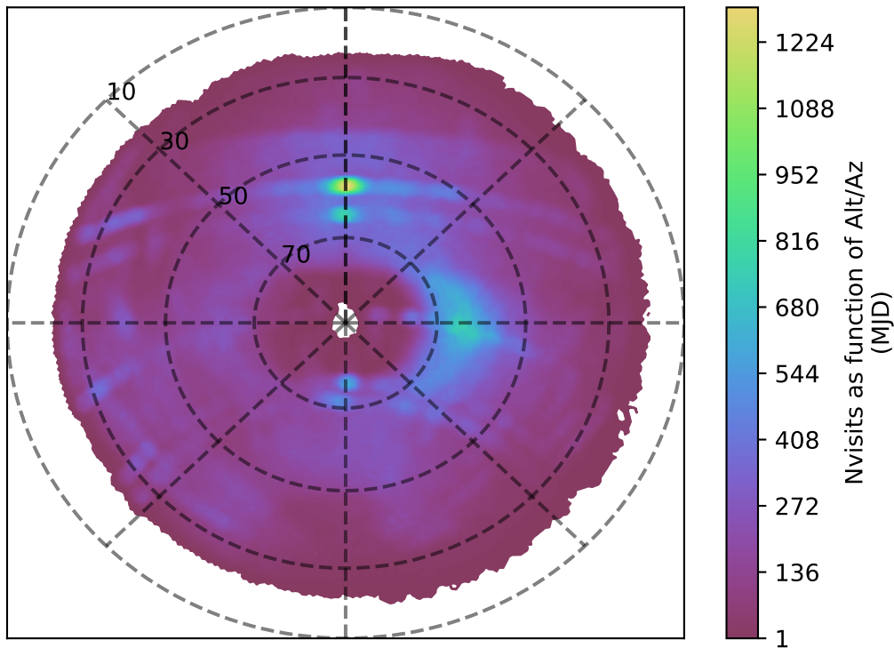
too_elab_r64_d3_gz_v3.4_10yrs g band: Nvisits as function of Alt/Az
