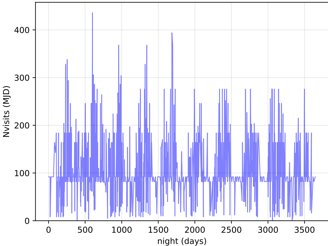
too_elab_r64_d3_gz_v3.4_10yrs DDF: Nvisits
