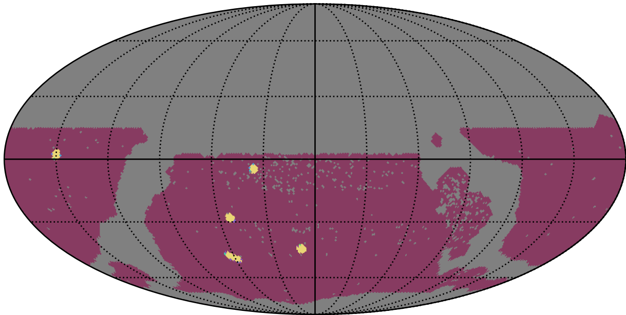
too_elab_r64_d3_gz_v3.4_10yrs WFD: NumberOfQuickRevisits
