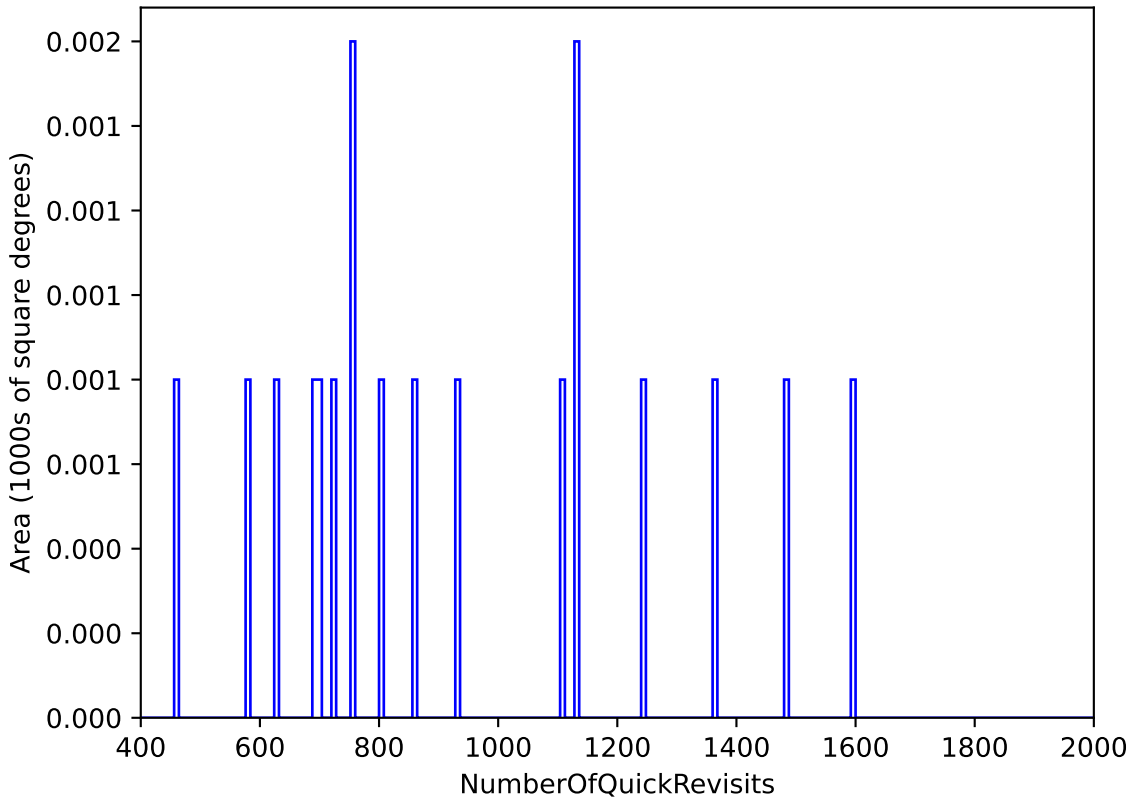
too_elab_r64_d3_gz_v3.4_10yrs WFD: NumberOfQuickRevisits
