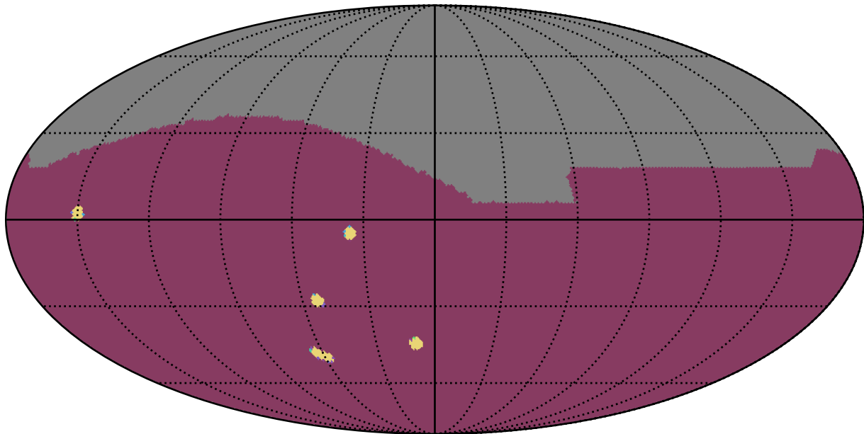
too_elab_r64_d3_gz_v3.4_10yrs All sky: NumberOfQuickRevisits
