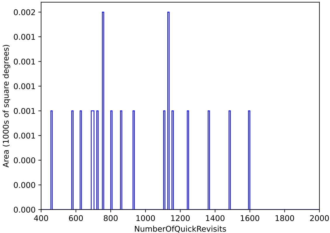
too_elab_r64_d3_gz_v3.4_10yrs All sky: NumberOfQuickRevisits
