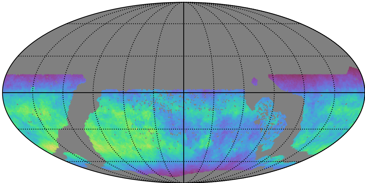
too_elab_r64_d3_gz_v3.4_10yrs WFD z band: Normalized Teff
