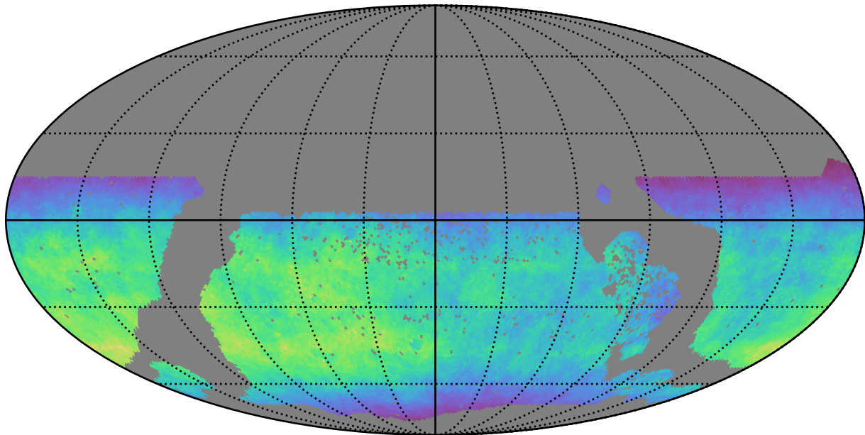
too_elab_r64_d3_gz_v3.4_10yrs WFD y band: Normalized Teff
