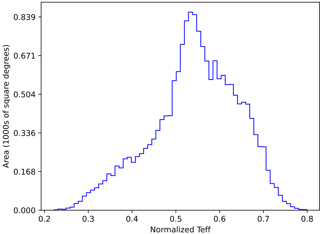
too_elab_r64_d3_gz_v3.4_10yrs WFD y band: Normalized Teff
