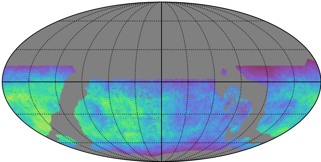
too_elab_r64_d3_gz_v3.4_10yrs WFD u band: Normalized Teff
