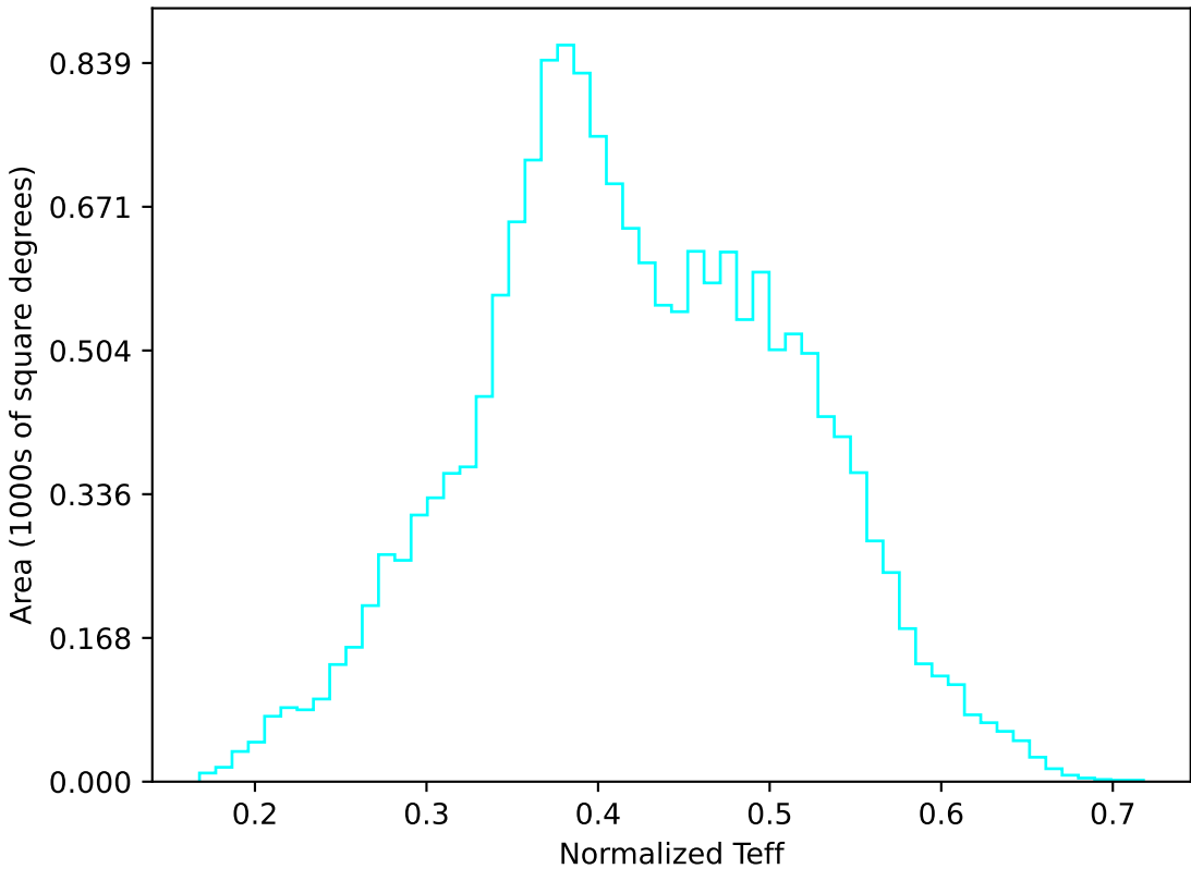
too_elab_r64_d3_gz_v3.4_10yrs WFD u band: Normalized Teff
