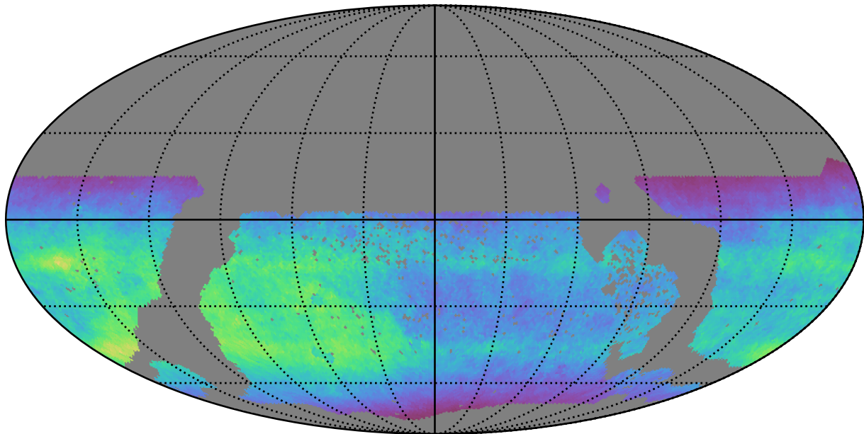
too_elab_r64_d3_gz_v3.4_10yrs WFD i band: Normalized Teff
