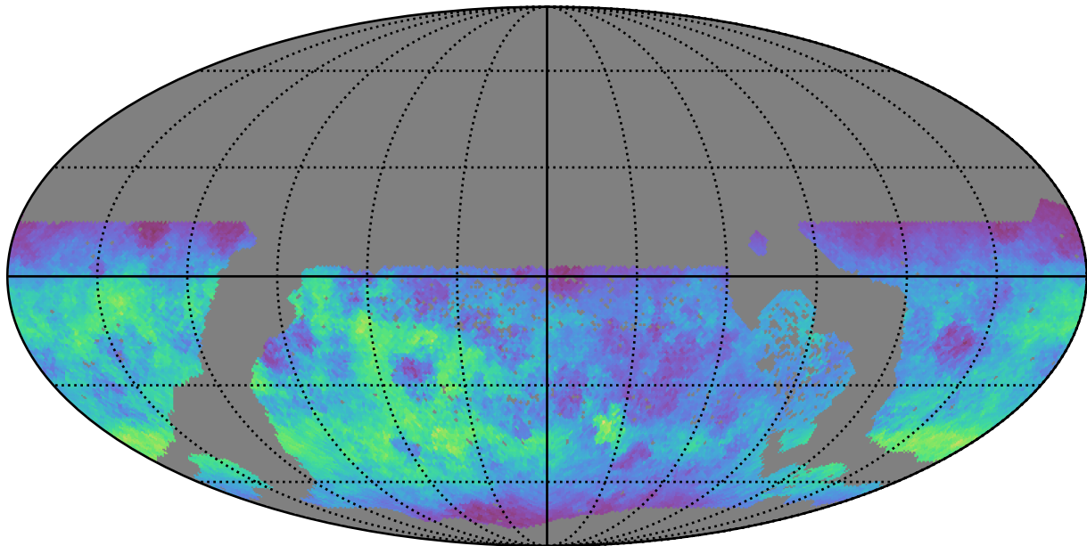
too_elab_r64_d3_gz_v3.4_10yrs WFD g band: Normalized Teff
