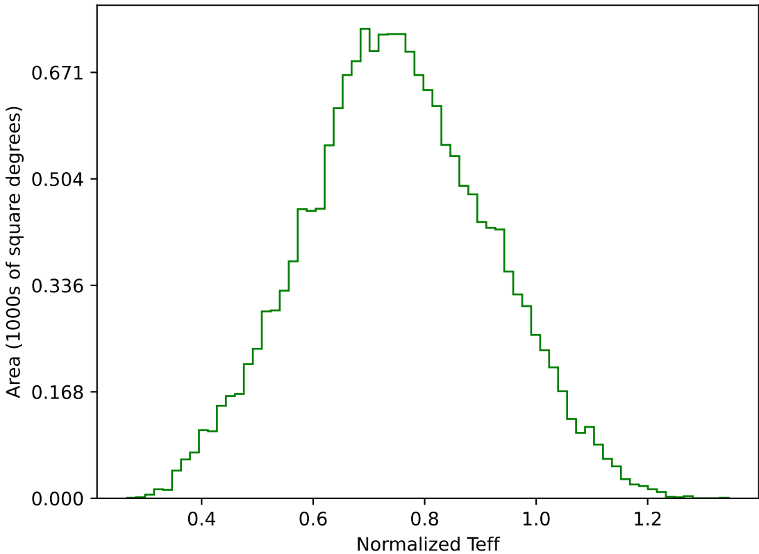
too_elab_r64_d3_gz_v3.4_10yrs WFD g band: Normalized Teff
