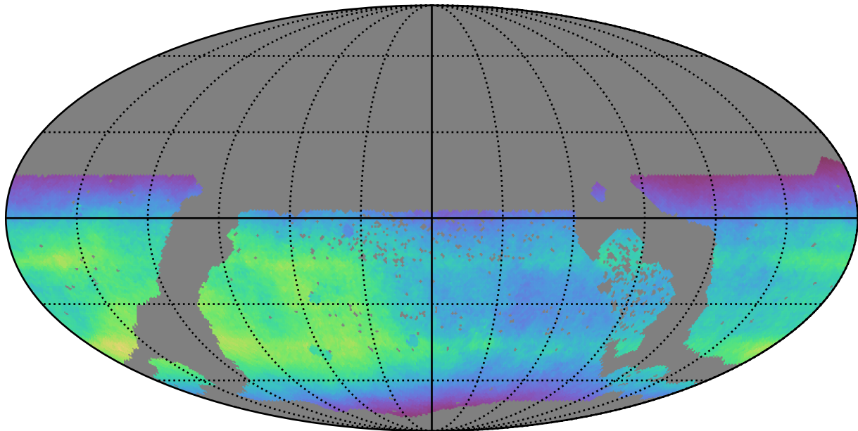
too_elab_r64_d3_gz_v3.4_10yrs WFD all bands: Normalized Teff
