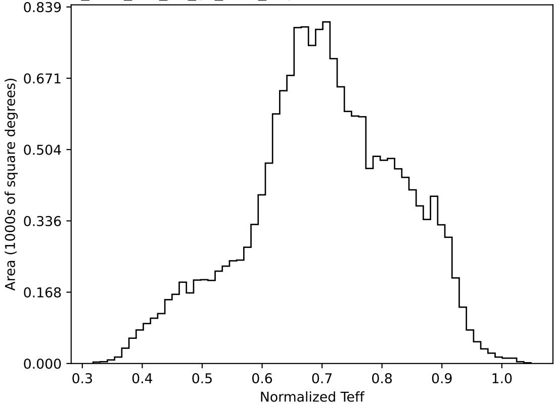
too_elab_r64_d3_gz_v3.4_10yrs WFD all bands: Normalized Teff
