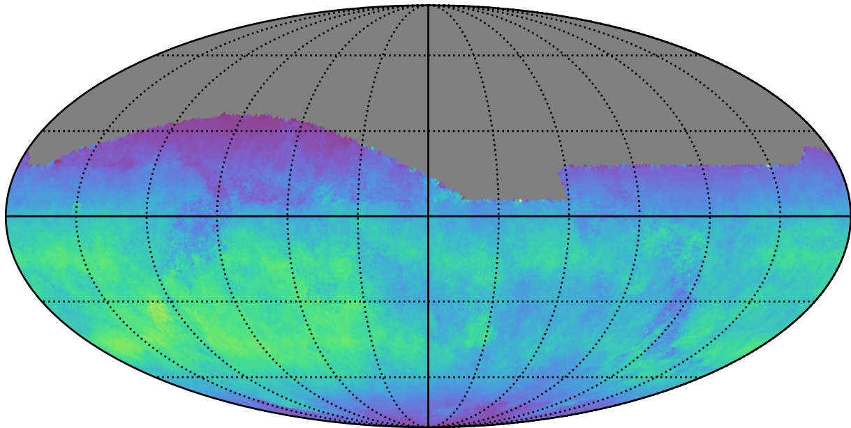
too_elab_r64_d3_gz_v3.4_10yrs All sky z band: Normalized Teff
