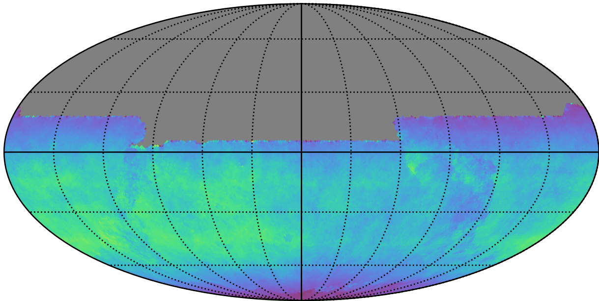
too_elab_r64_d3_gz_v3.4_10yrs All sky y band: Normalized Teff
