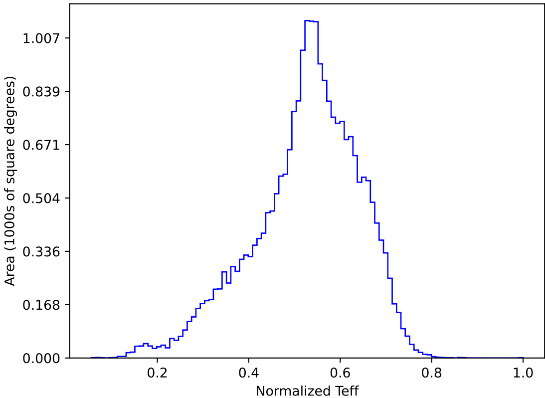
too_elab_r64_d3_gz_v3.4_10yrs All sky y band: Normalized Teff
