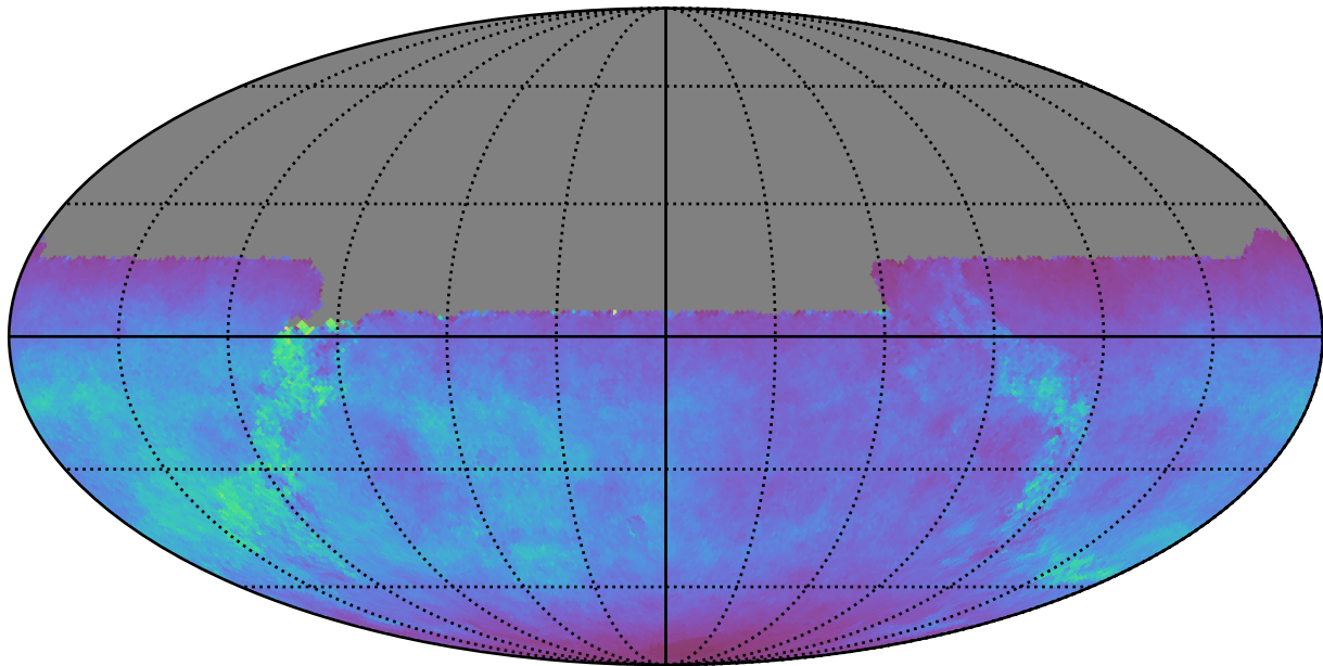
too_elab_r64_d3_gz_v3.4_10yrs All sky u band: Normalized Teff
