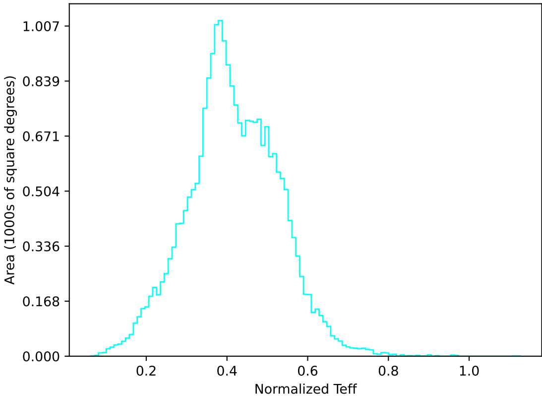
too_elab_r64_d3_gz_v3.4_10yrs All sky u band: Normalized Teff
