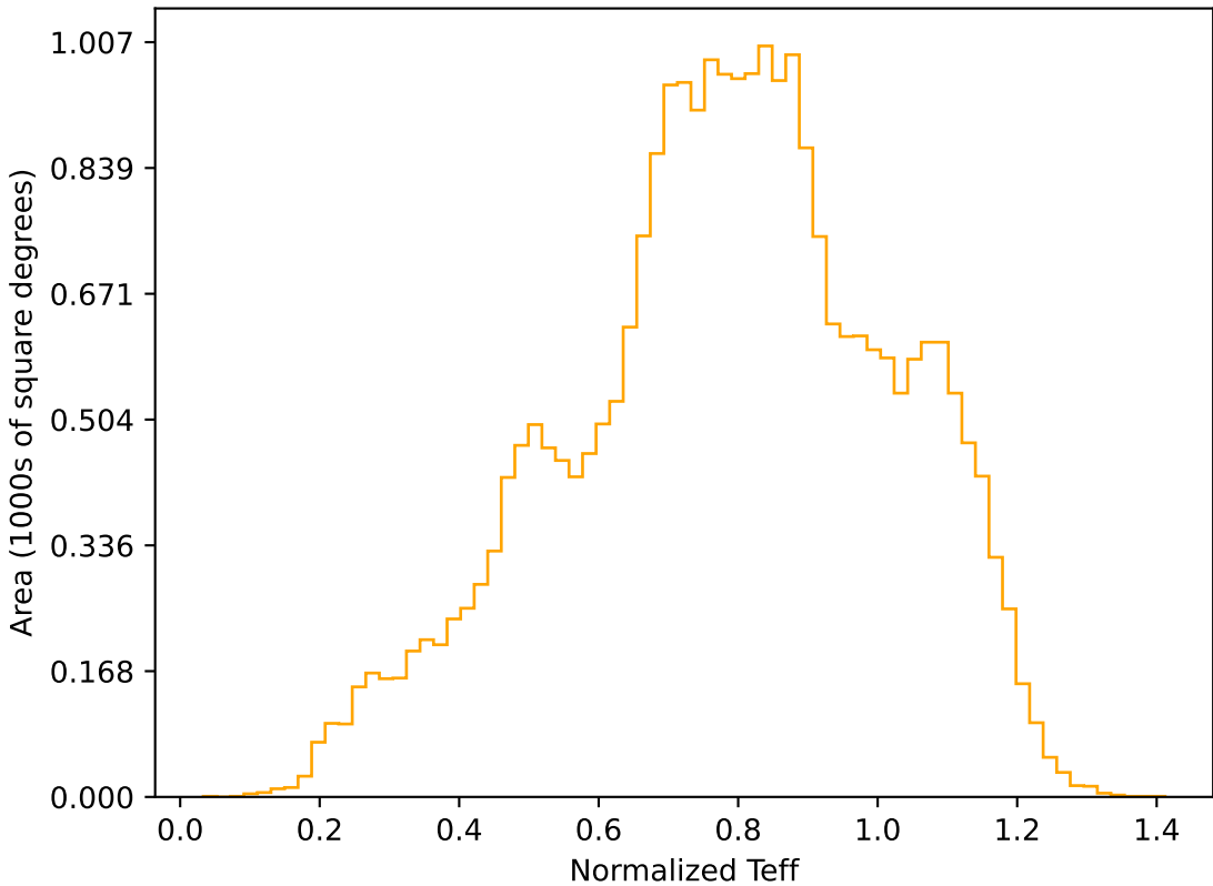
too_elab_r64_d3_gz_v3.4_10yrs All sky r band: Normalized Teff
