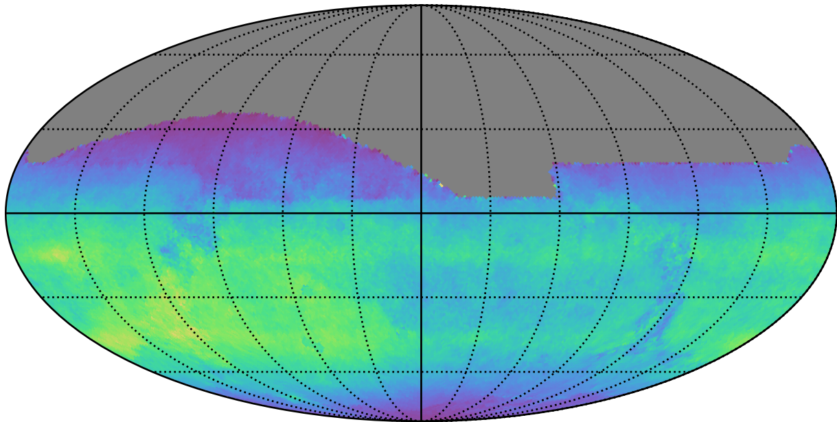
too_elab_r64_d3_gz_v3.4_10yrs All sky i band: Normalized Teff
