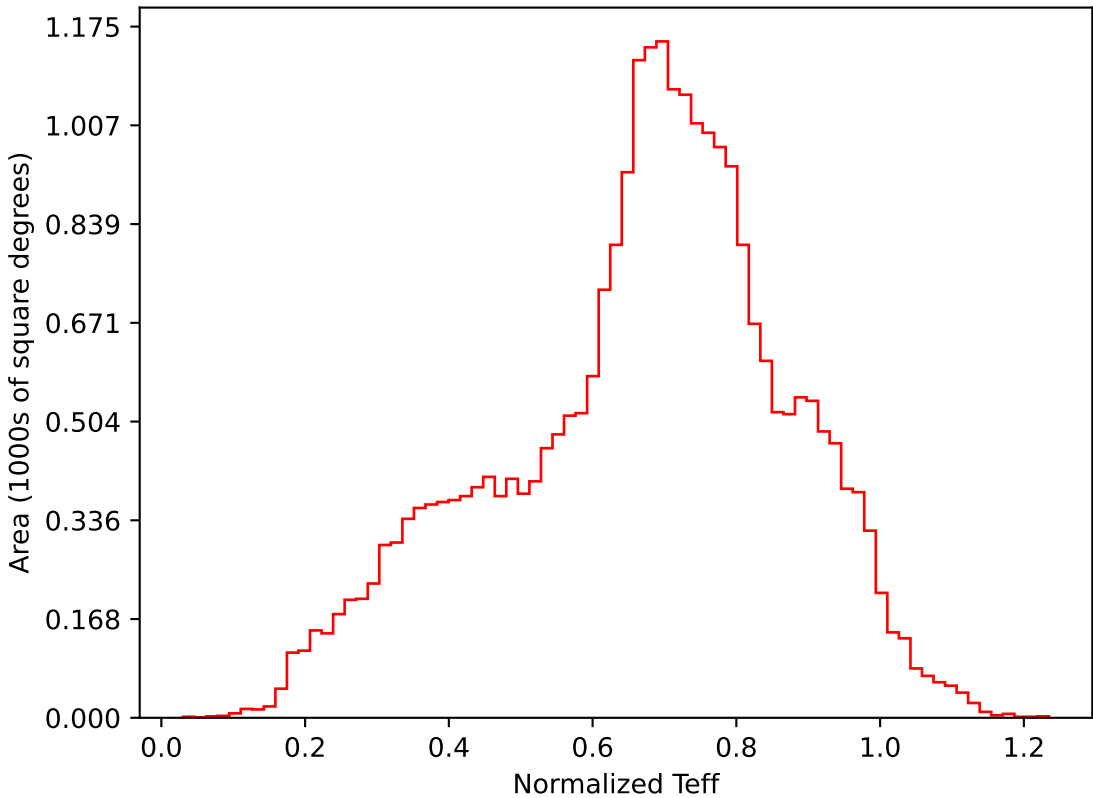
too_elab_r64_d3_gz_v3.4_10yrs All sky i band: Normalized Teff
