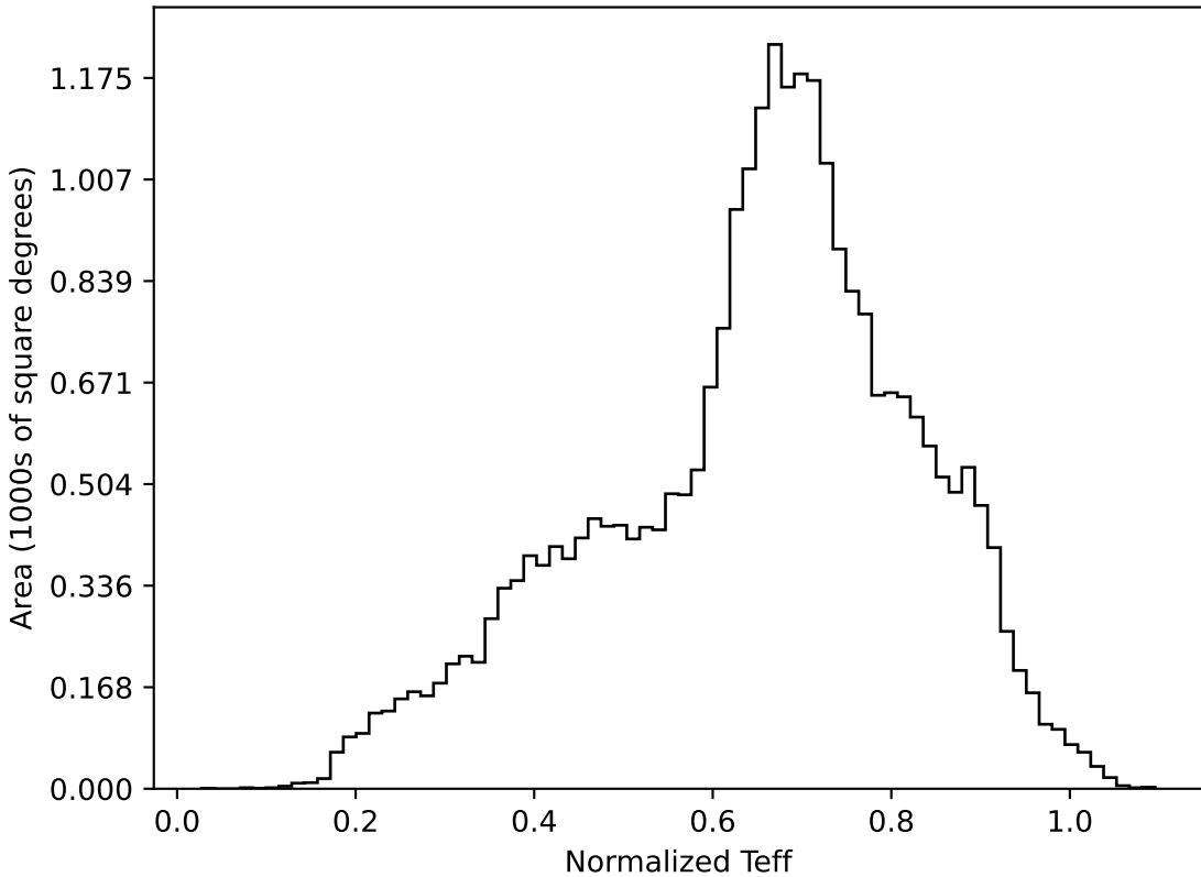
too_elab_r64_d3_gz_v3.4_10yrs All sky all bands: Normalized Teff
